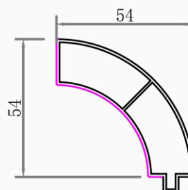
HT-061 (Internal corner)
