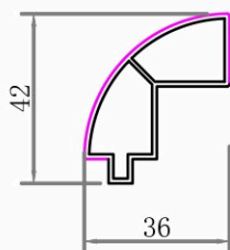
HT-059 (External corner)
